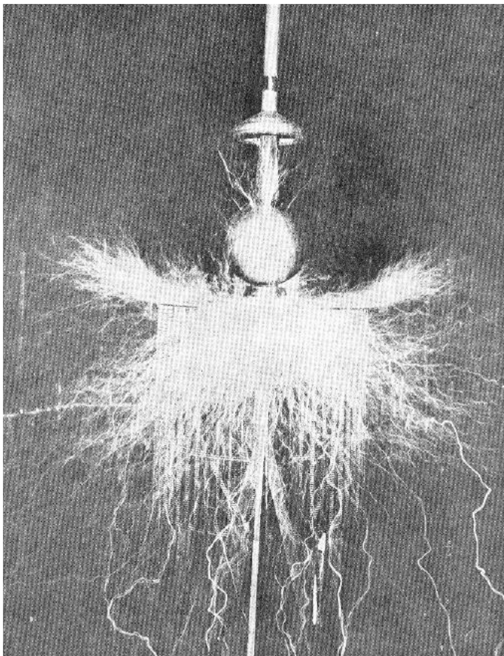
Fig. 9: Experiment to illustrate the capacity on the oscillator for creating a great electrical movement.
