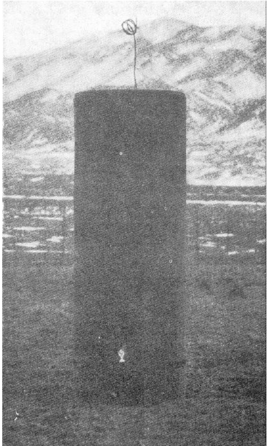
Fig. 4: Experiment to illustrate the transmission of electrical energy through the Earth without wire.
