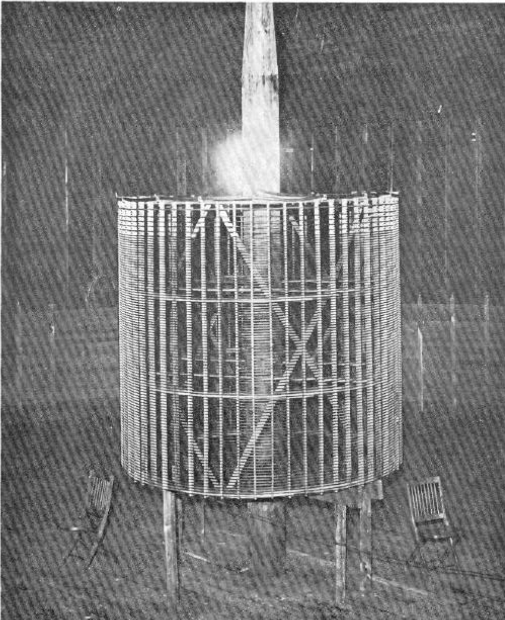
Fig. 3. Experiment to illustrate the supplying of electrical energy through a single wire without return.
