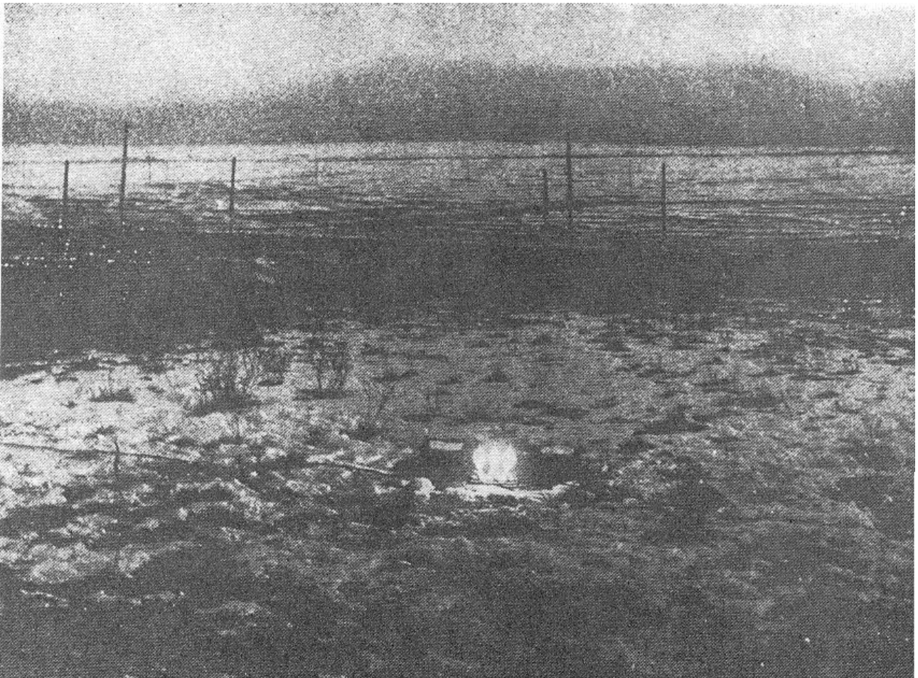
Fig. 7: Experiment to illustrate an inductive effect of an electrical oscillator of great power.
