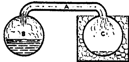
The "cryophros" is well known as a scientific toy, exemplifying also the principle of refrigerating machinery.
